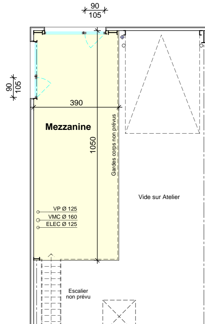
PLAN MEZZANINE
