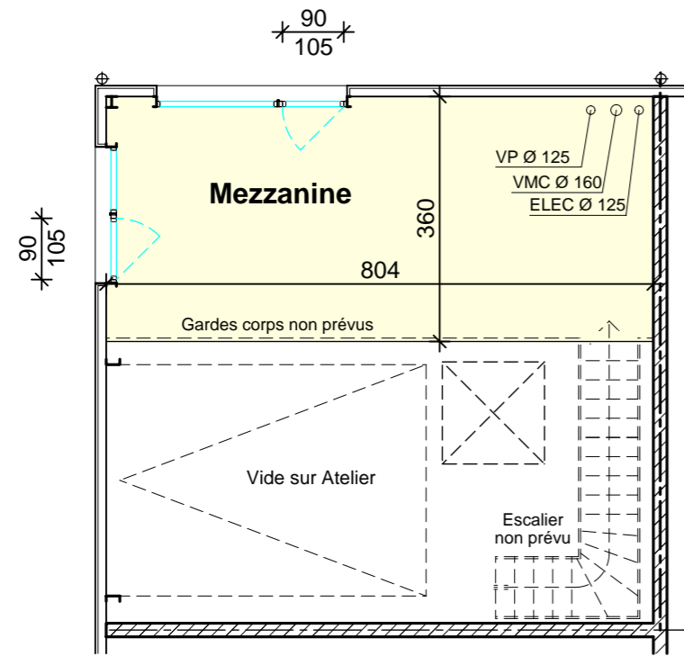
PLAN MEZZANINE
