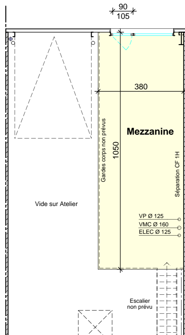
PLAN MEZZANINE
