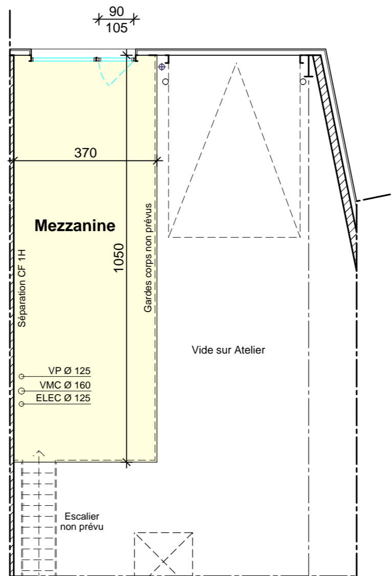
PLAN MEZZANINE
