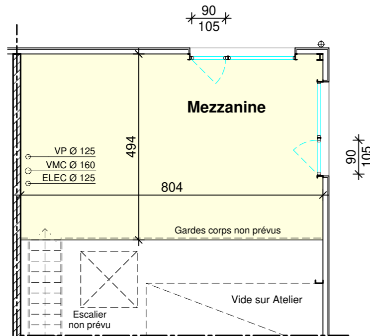
PLAN MEZZANINE
