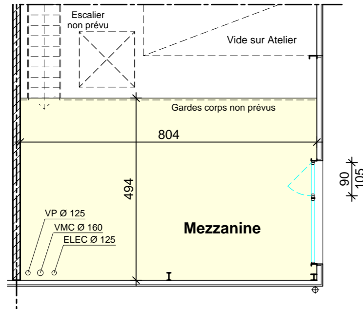
PLAN MEZZANINE
