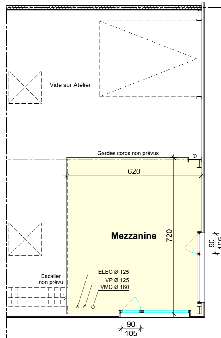
PLAN MEZZANINE
