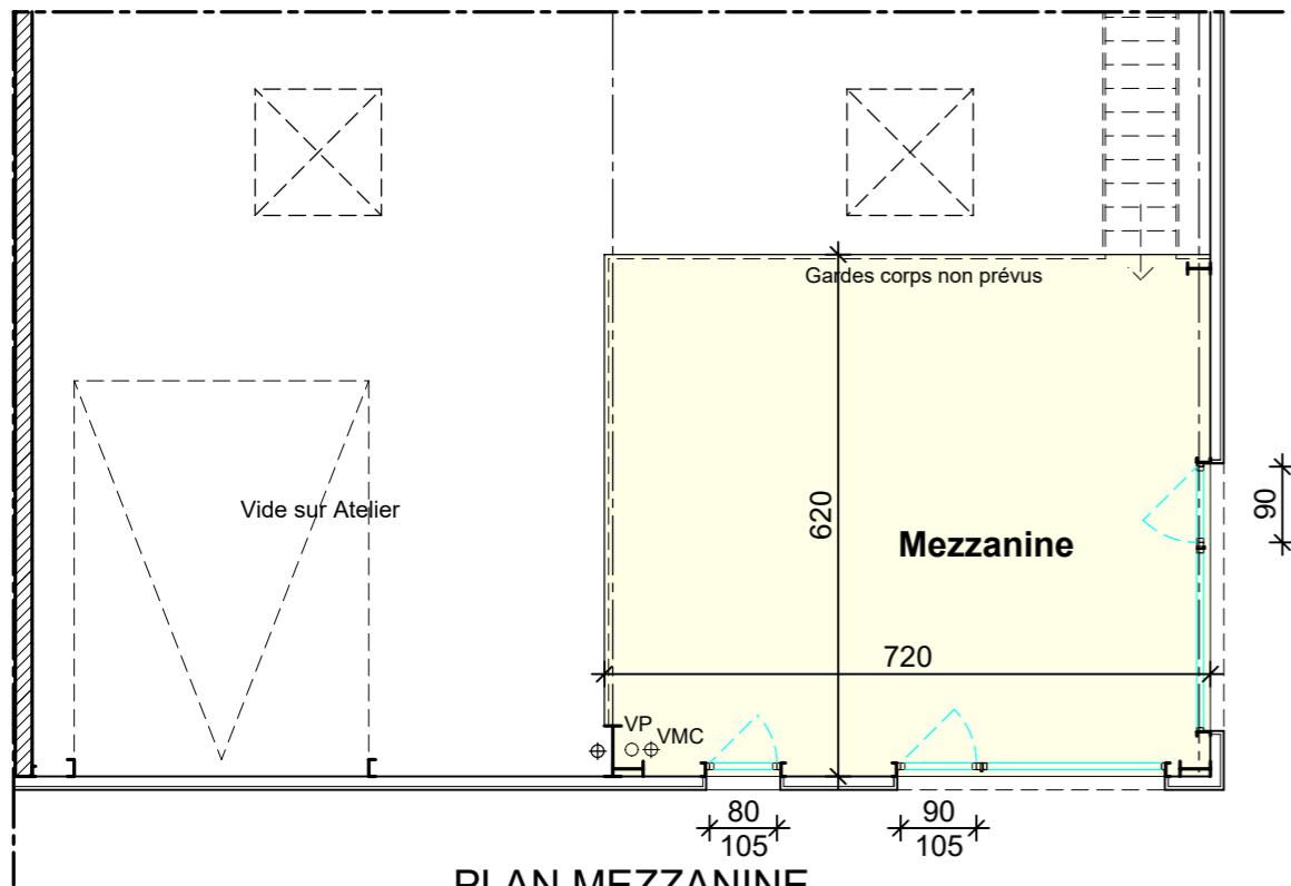
PLAN MEZZANINE
