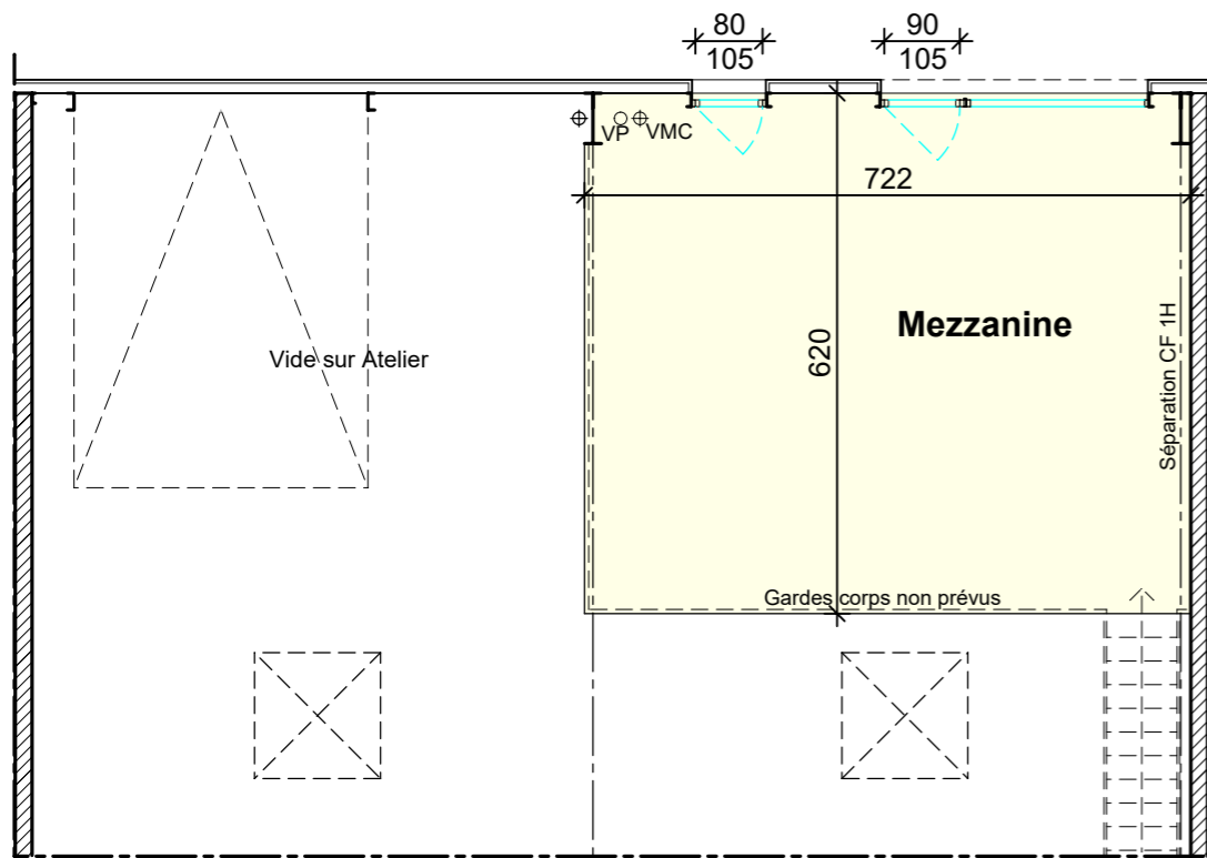
PLAN MEZZANINE
