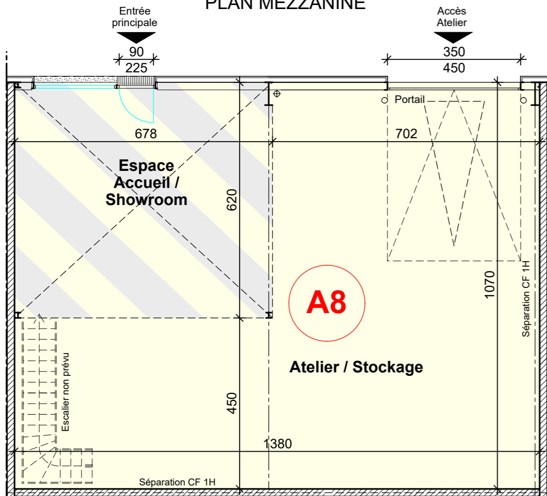
PLAN MEZZANINE
