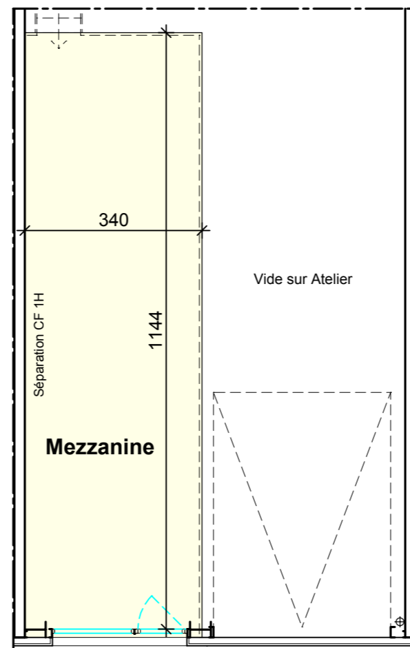
PLAN MEZZANINE
