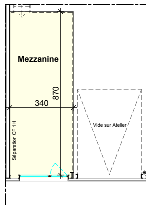
PLAN MEZZANINE
