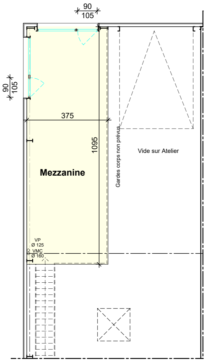
PLAN MEZZANINE
