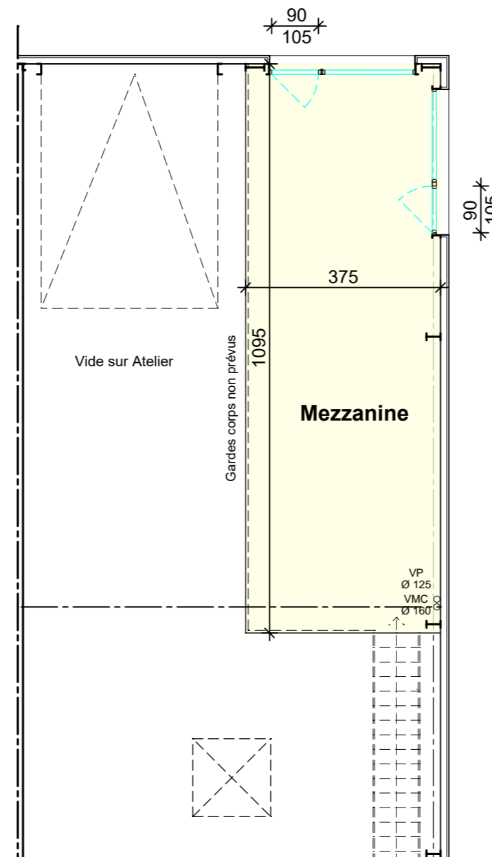
PLAN MEZZANINE
