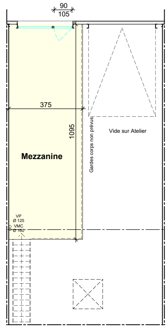
PLAN MEZZANINE
