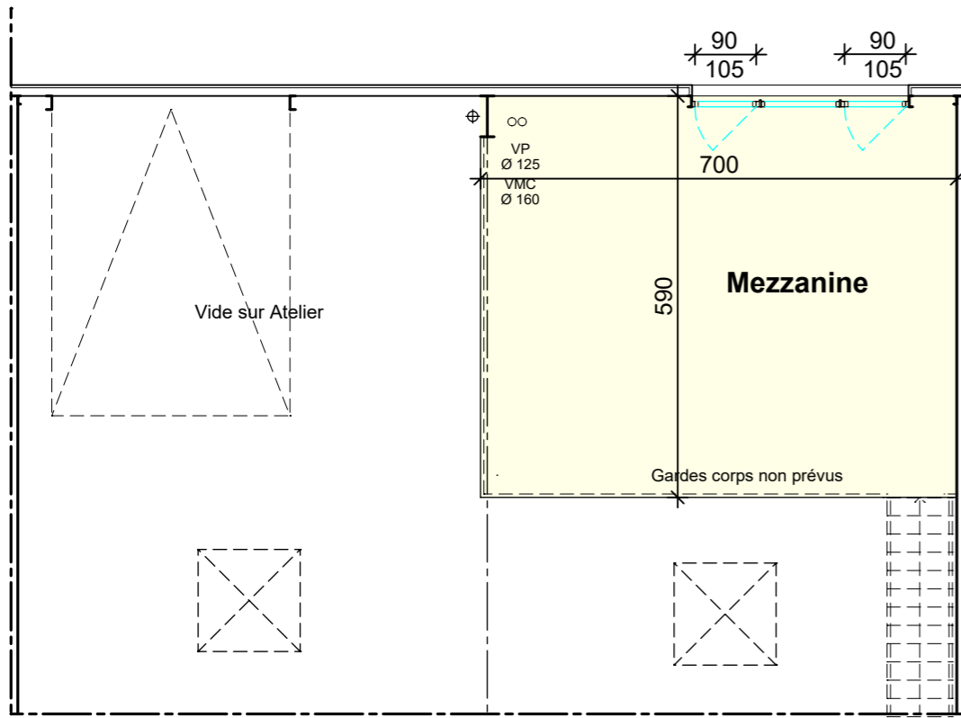
PLAN MEZZANINE
