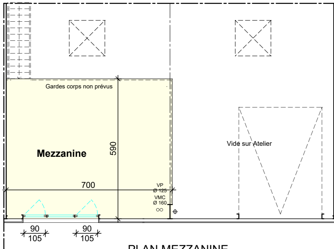
PLAN MEZZANINE
