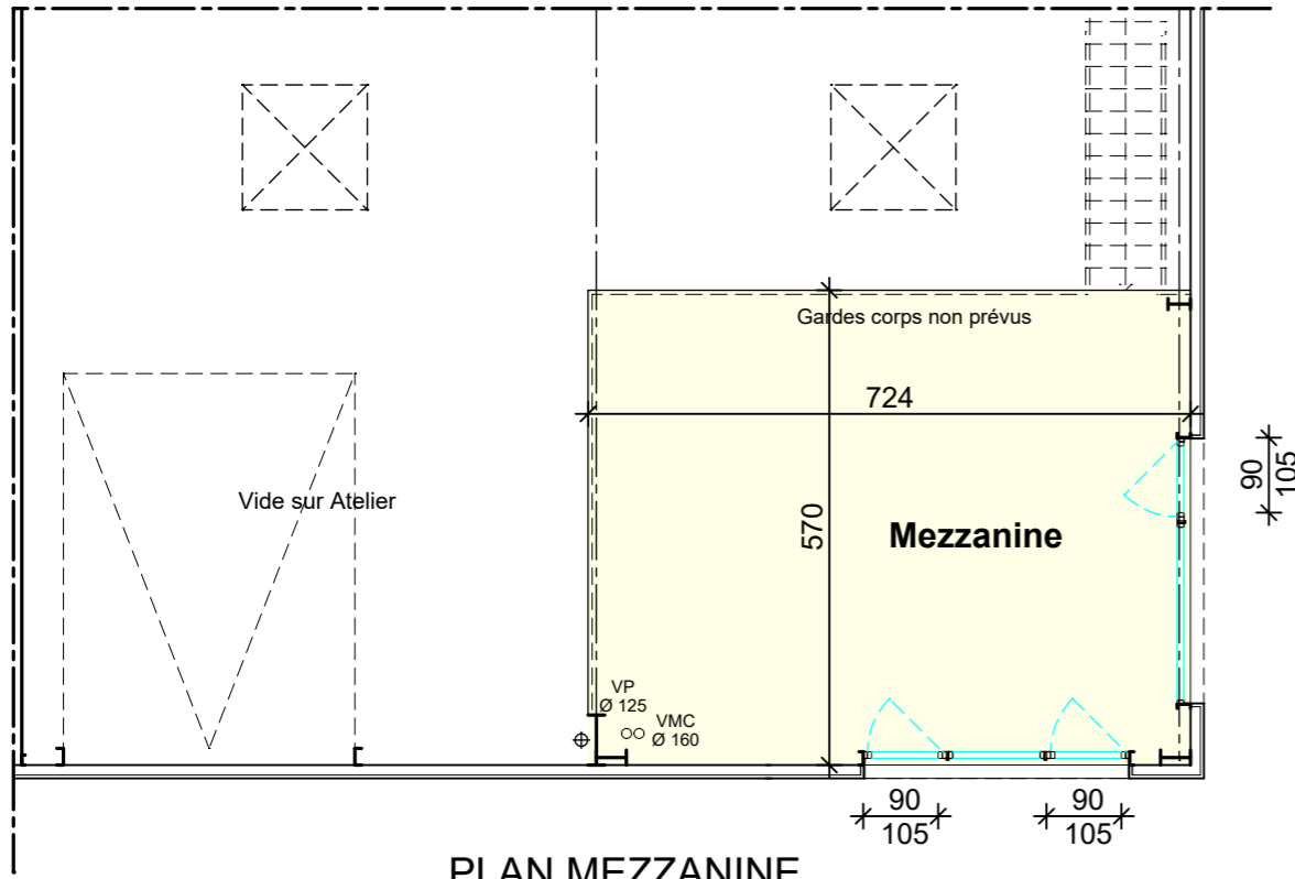
PLAN MEZZANINE
