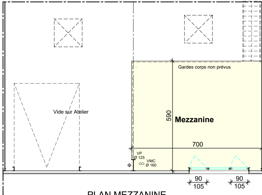
PLAN MEZZANINE
