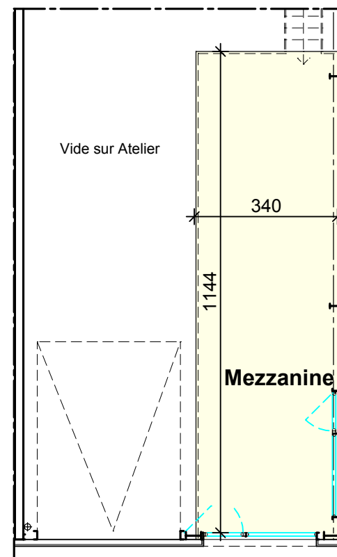
PLAN MEZZANINE
