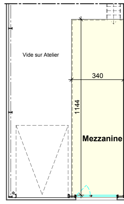
PLAN MEZZANINE
