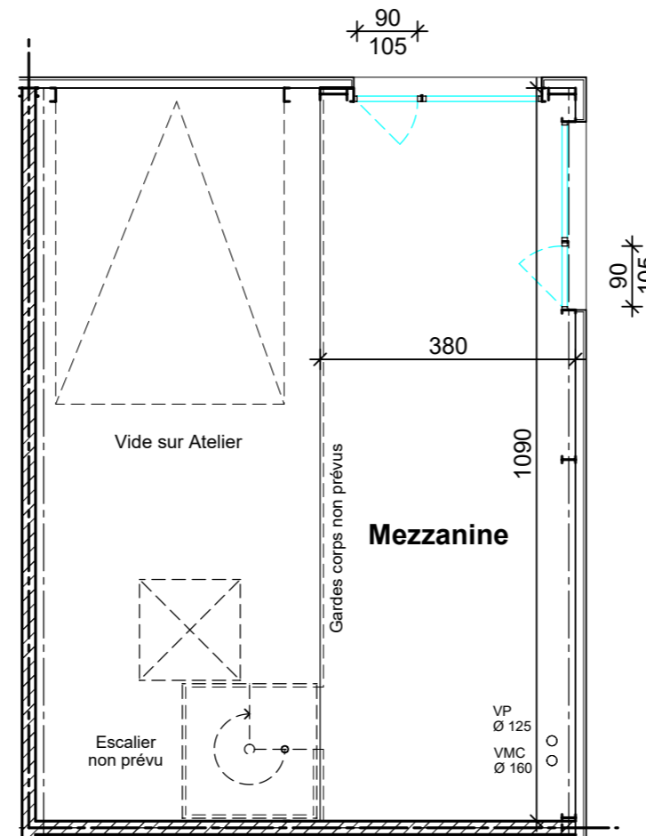
PLAN MEZZANINE
