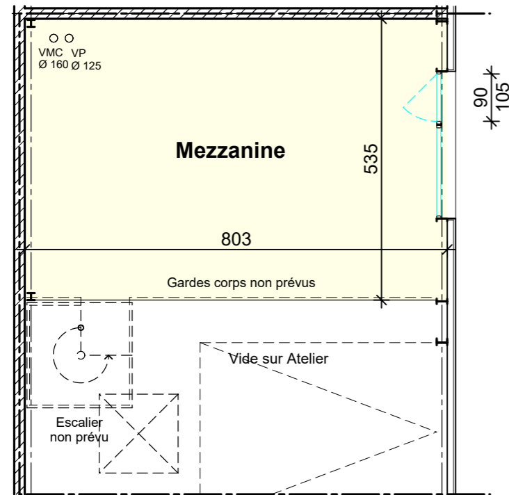
PLAN MEZZANINE
