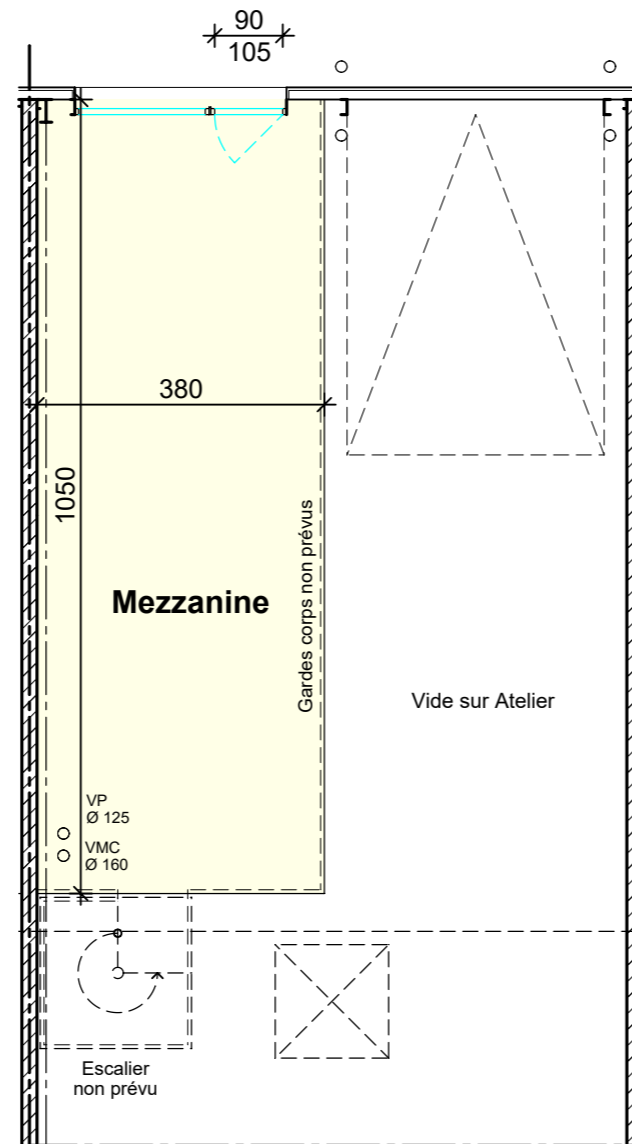
PLAN MEZZANINE
