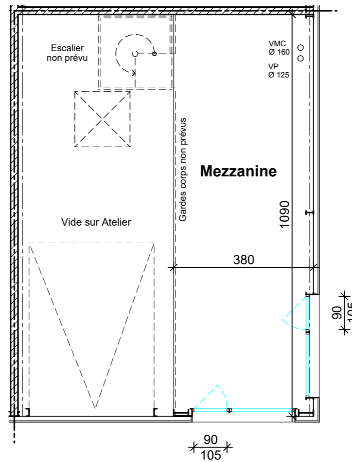
PLAN MEZZANINE
