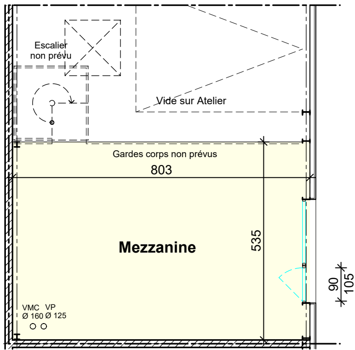
PLAN MEZZANINE
